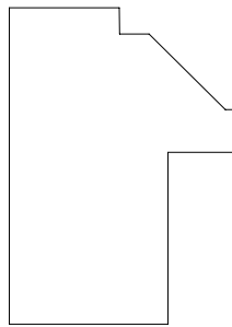
BACKBAND 615019 1 1/2" x 1 1/8" 7/8" THROAT
