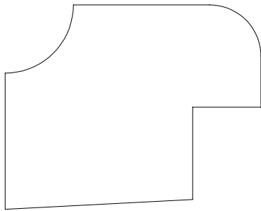
BACKBAND 615020 1 1/2" X 1 7/8" WITH 3/4" THROAT
