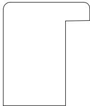
BACKBAND 611311 1 1/8" X 7/8" 1/4" X 7/8" THROAT
