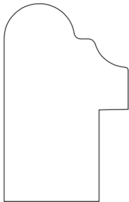
BACK BAND 61753 1 1/8" X 1 3/4"
