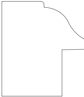
BACKBAND 61691 1 5/8" x 1 1/2" 7/8" THROAT
