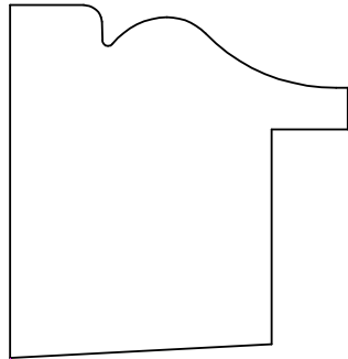
BACK BAND 61135 1 3/16" X 1 1/8"
