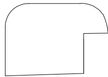
BACKBAND 6081 3/4" X 1 1/16" (7/16" THROAT)
