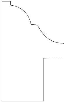
BACKBAND 61755 1 3/4" x 1 1/8" 3/8" x 3/4" THROAT
