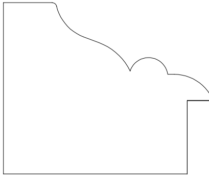
BACKBAND 6213 1 3/4" X 2 1/8" 1/4" X 3/4" THROAT
