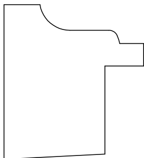
BACK BAND 61255 1 1/4" X 1 1/8"
