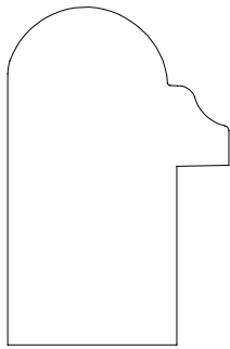
BACKBAND 61635 1 5/8" X 1 1/16" (55/64" THROAT)
