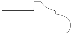
BACKBAND 61564 1 17/32" X 21/32" (25/32" KNOTCH)
