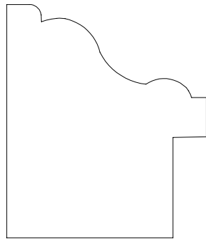
BACKBAND 61759 1 3/4" X 1 1/2" ( 3/4" KNOTCH )
