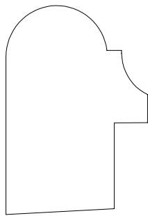
BACKBAND 6156 1 9/16" X 1 1/16" 1/4" X 11/16" THROAT
