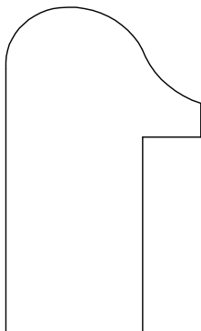
BACK BAND 61252 1 1/4" X 3/4"
