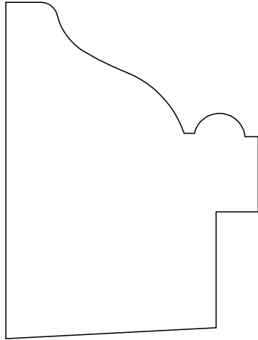
BACK BAND 62002 2" X 1 1/2"
