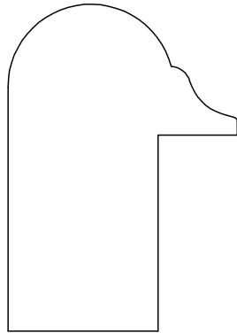
BACK BAND 61253 1 1/4" X 7/8"
