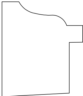
BACK BAND 61133 1 5/16 X 1 1/8"
