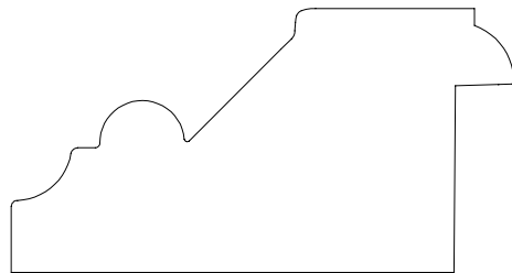
BACKBAND 6238 1 1/4" X 2 3/8" 1/4" X 7/8" THROAT
