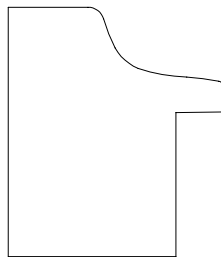
BACKBAND 61191 1 1/4" x 1 1/8" 1/4" x 3/4" THROAT
