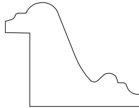
BACKBAND 613814 1 1/16" X 1 3/8" 1/4" X 3/4" THROAT
