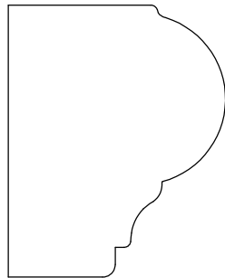
NOSING 9157 1 9/16" X 1 1/4"
